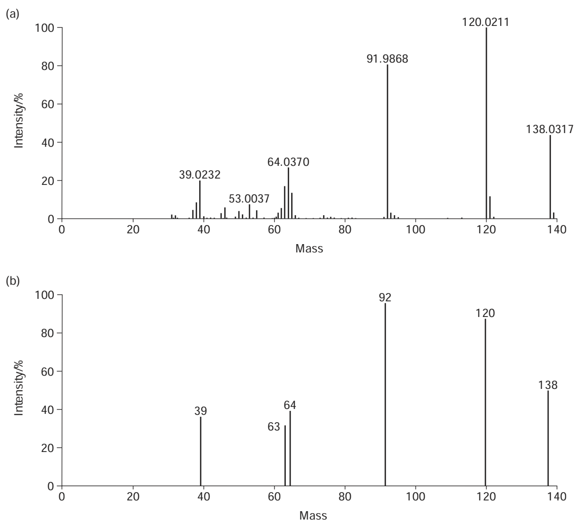
Figure 9 The mass spectrum of salicylic acid (a) high-resolution spectrum, (b) low-resolution spectrum. The relative heights are not the same as different experimental conditions have been used.
