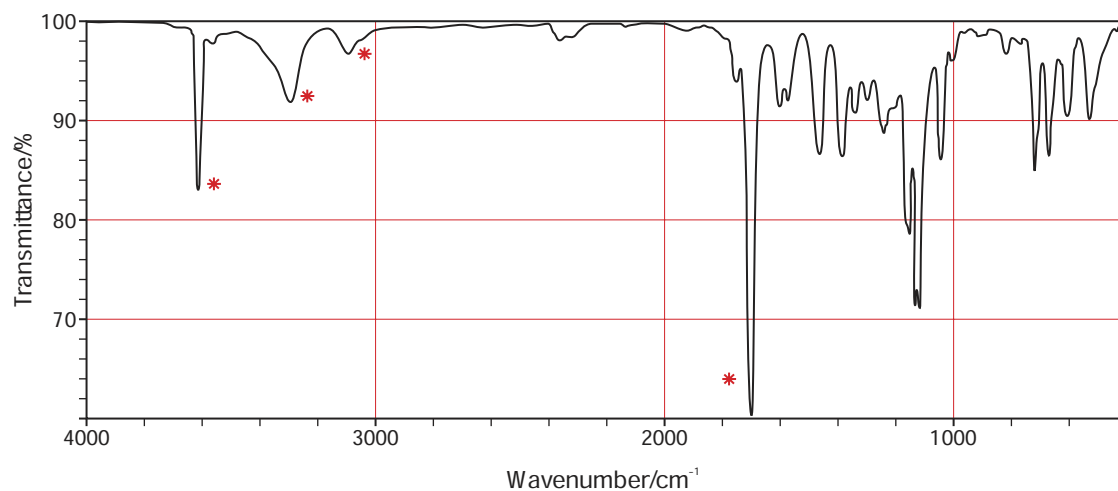
Figure 6 The i.r. spectrum of salicylic acid (in the gas phase).
