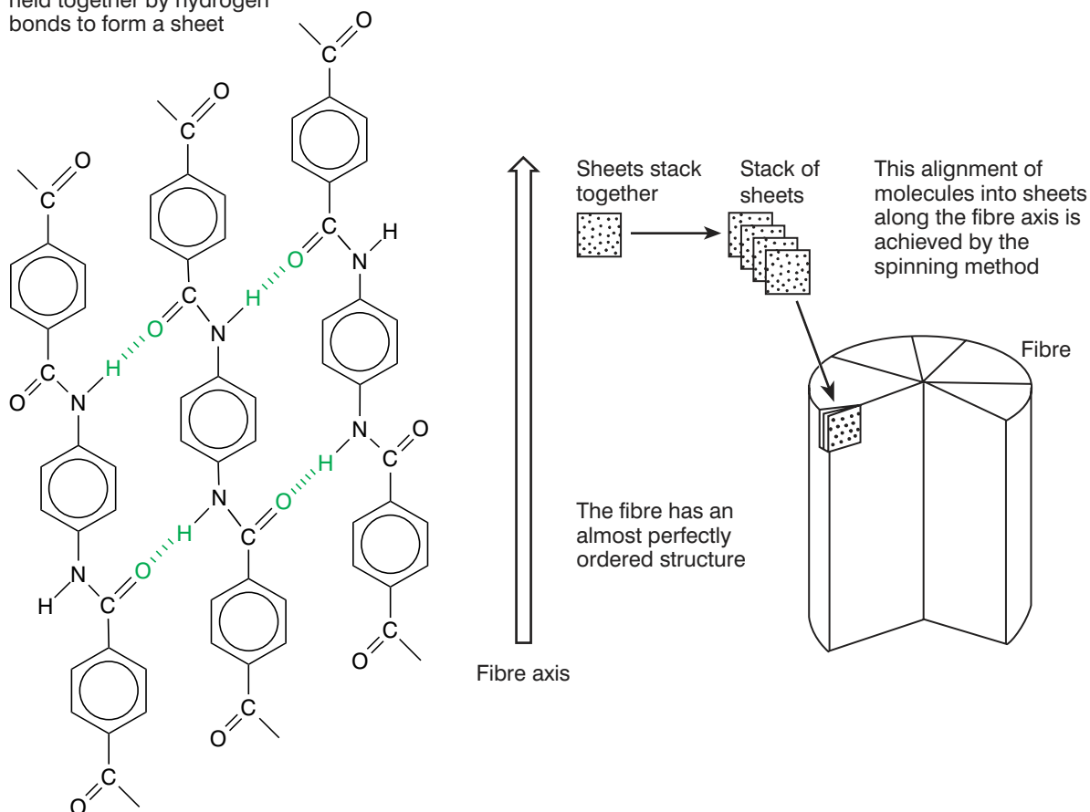
Figure 16 An illustration of the crystalline structure of Kevlar.
